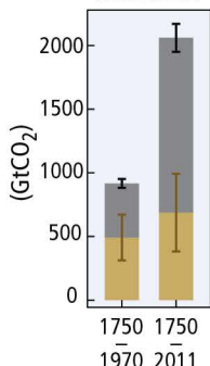
Cumulative CO 2 emissions
