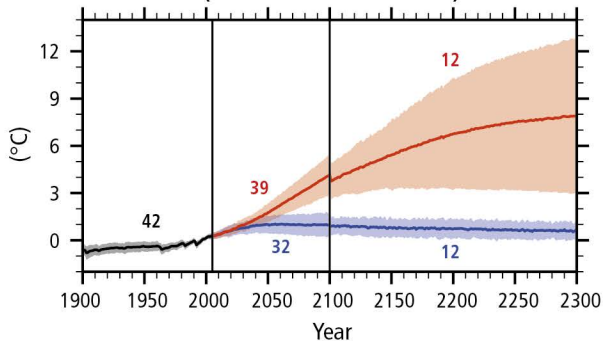
(b) Global average surface temperature change (relative to 1986–2005)
