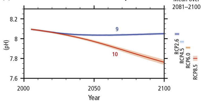
(e) Global surface ocean pH
