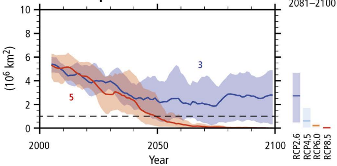
(c) Northern Hemisphere September sea ice extent
