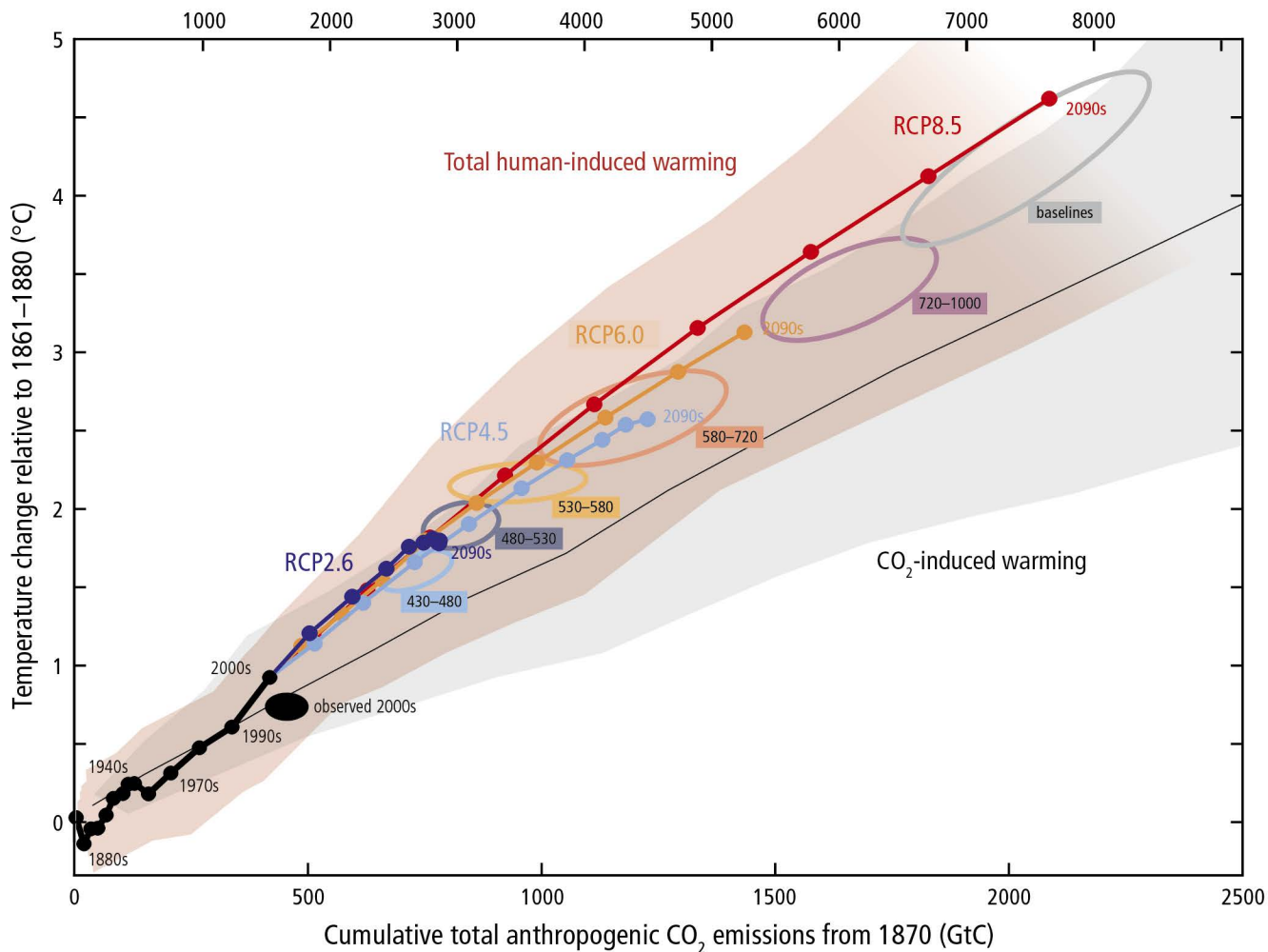
Cumulative total anthropogenic CO 2 emissions from 1870 (GtCO 2 )
