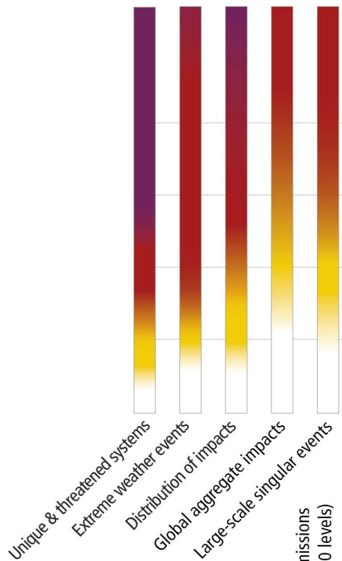
(a) Risks from climate change...
