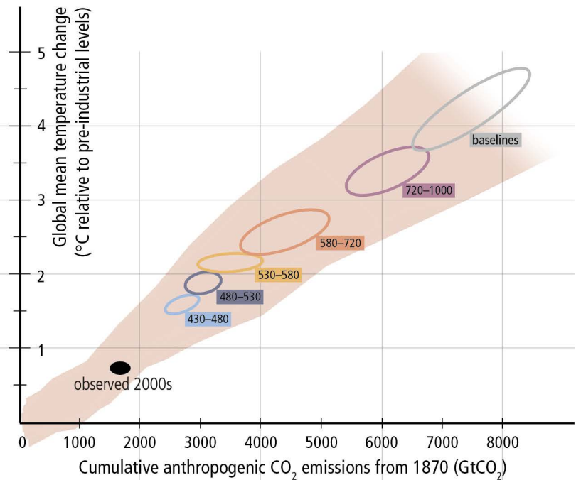
(b) ...depend on cumulative CO 2 emissions...
