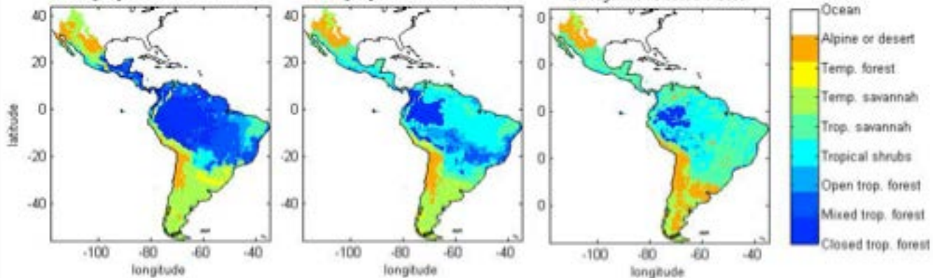
Natveg vegetation classes in 1951
